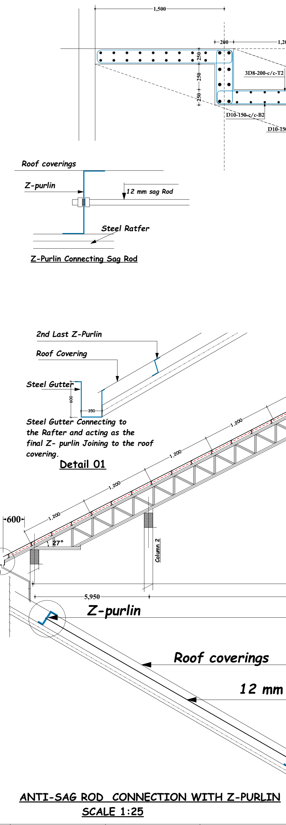
TERRACED DETAILS
