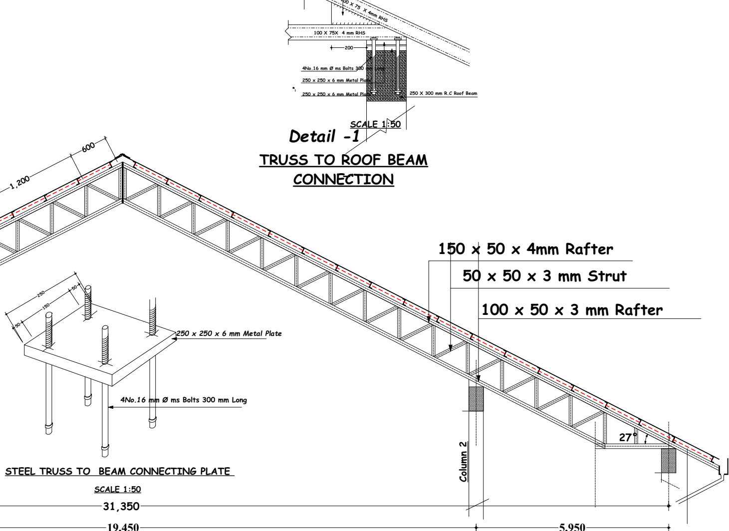
TYPICAL STEEL TRUSS A
