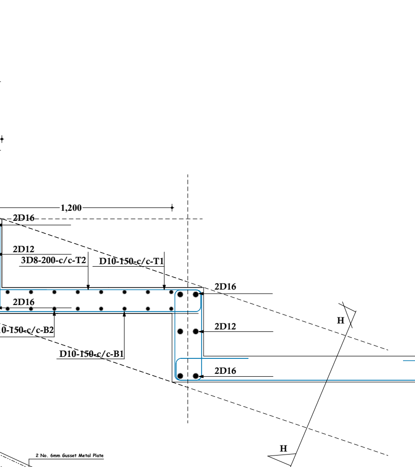
Detail -1 TRUSS TO ROOF BEAM CONNECTION
