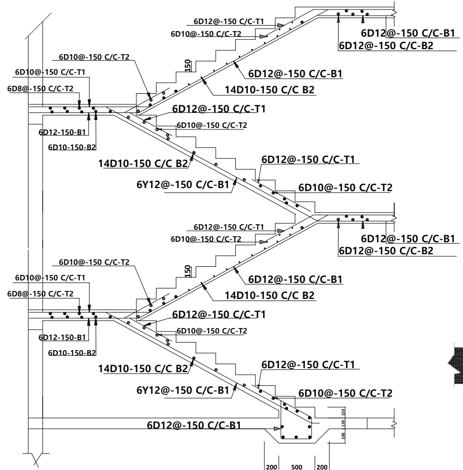
TYPICAL SECTION THROUGH STAIRCASE R.C. DETAILS FROM G.L. TO THE TERRACE FLOOR
