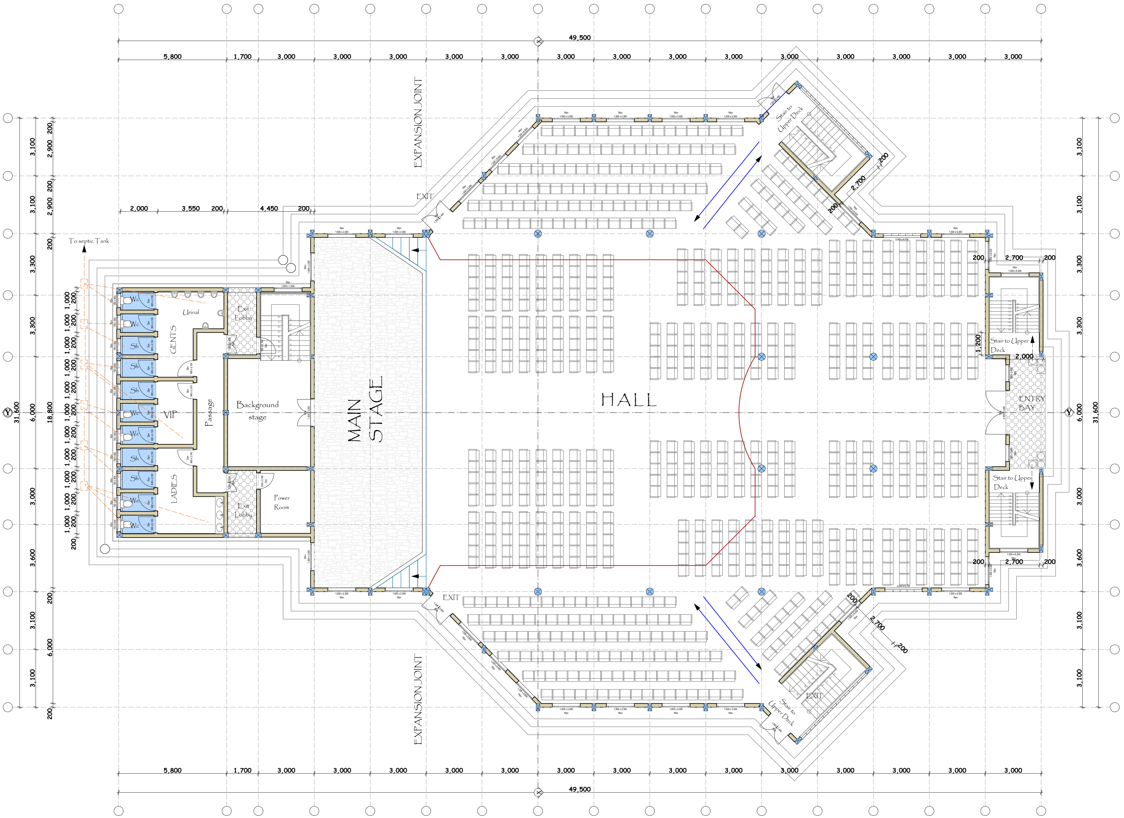
FLOOR PLAN LAYOUT
