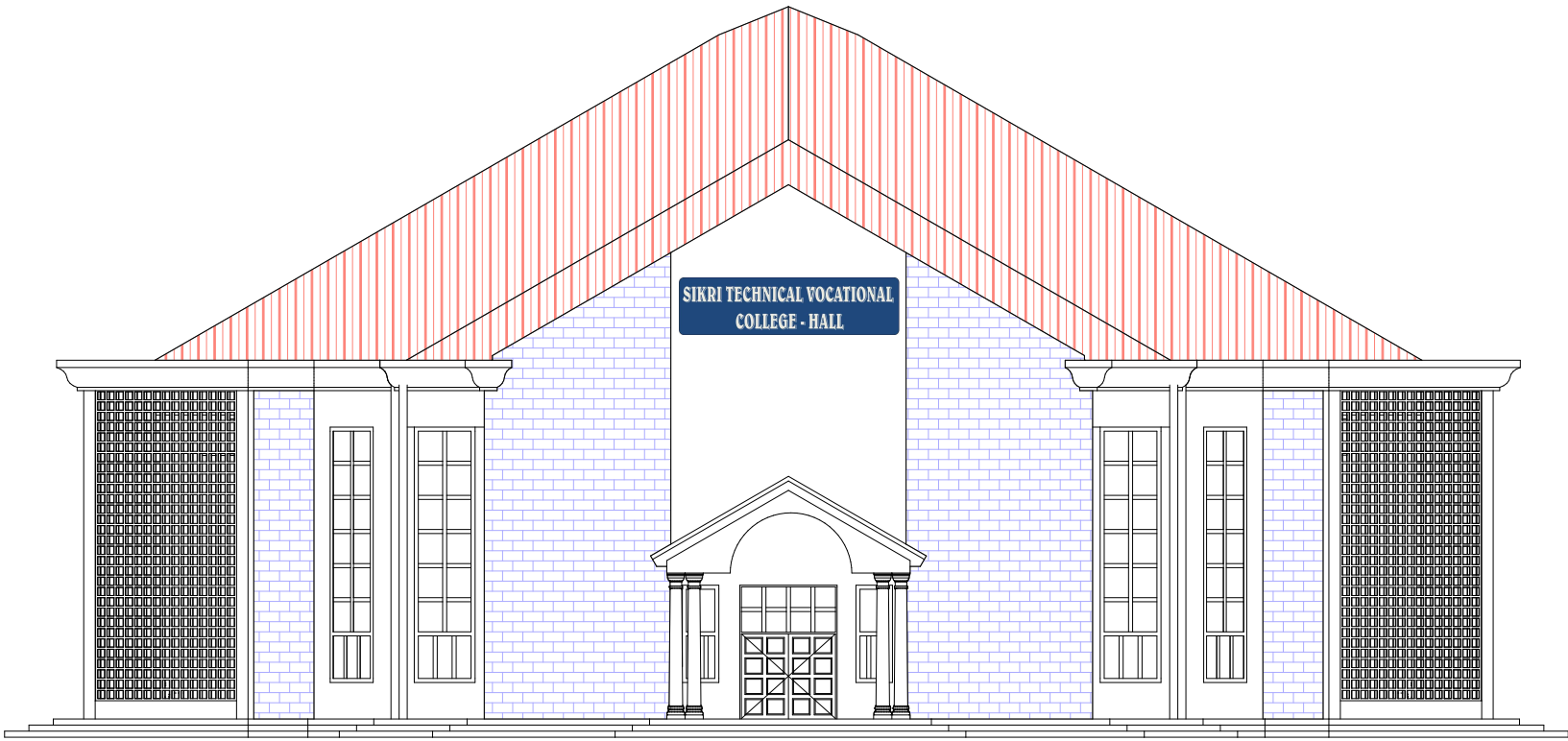
FRONT ELEVATION 01 SCALE 1:100
