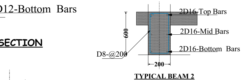
TYPICAL BEAM 2
