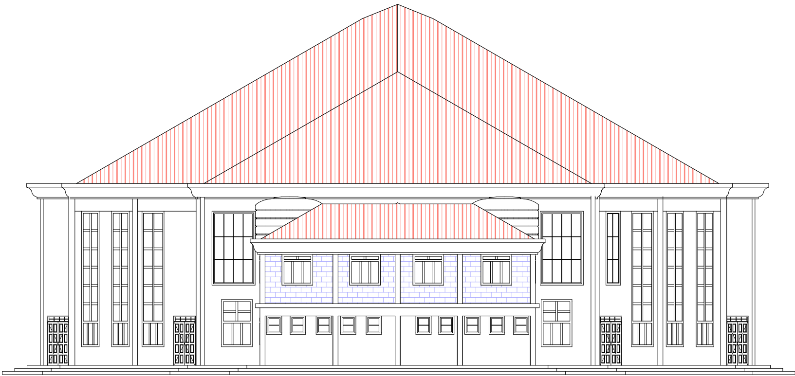
BACK ELEVATION 02 SCALE 1:100
